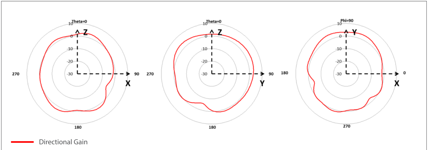
XZ-CUT
